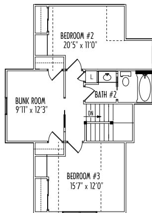
SECOND FLOOR PLAN 721 SQ. FT. LIVING
