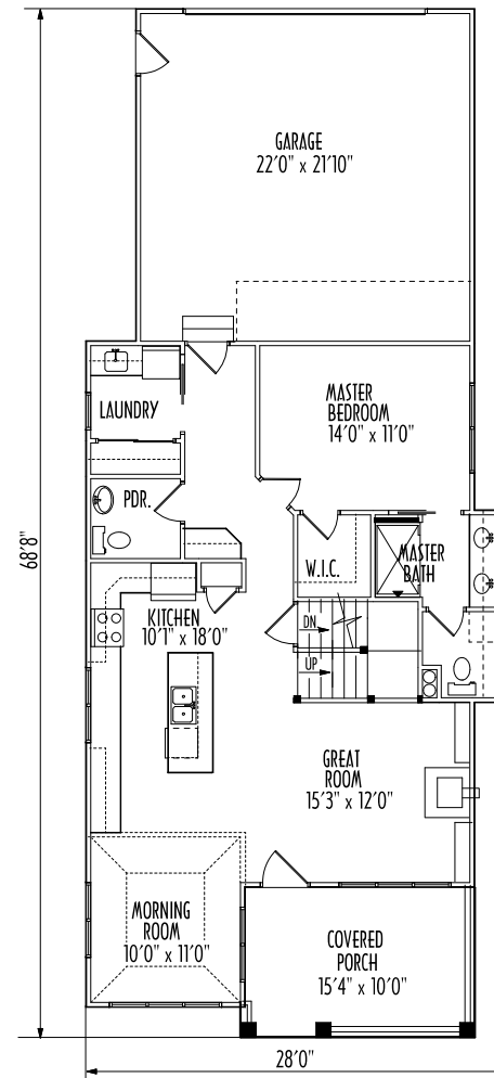
FIRST FLOOR PLAN 1061 SQ. FT. LIVING
